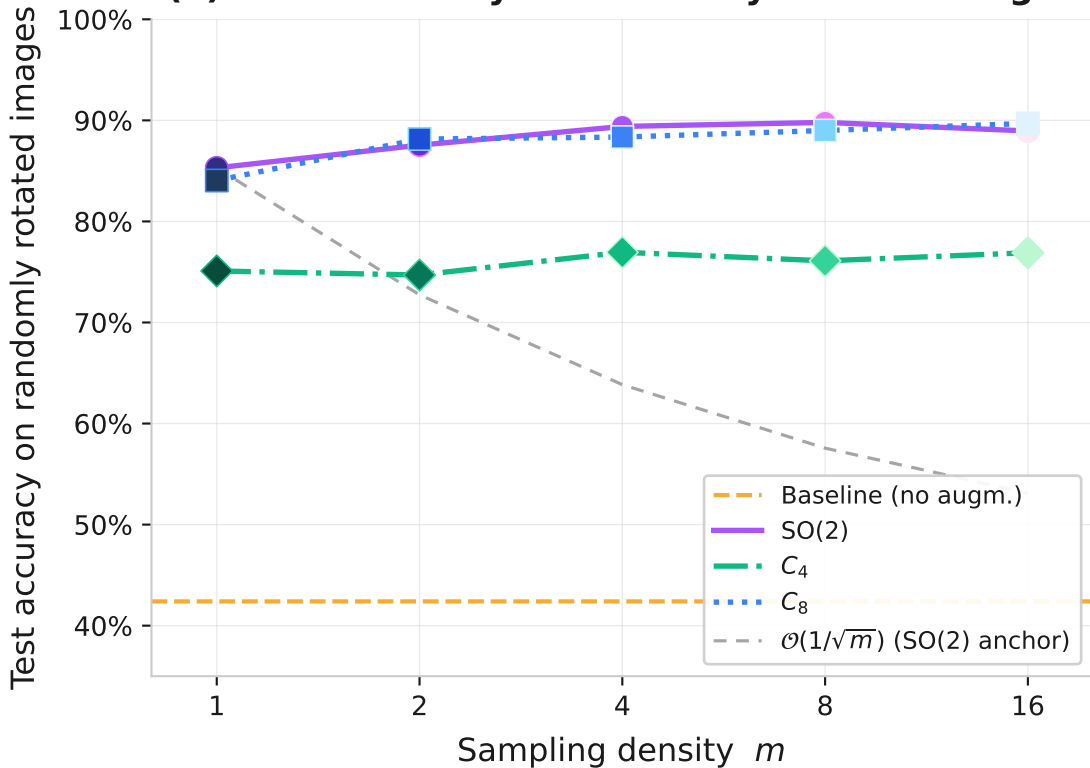
(a) Test accuracy on randomly rotated images
