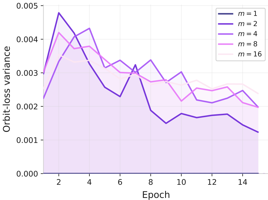
(a) SO(2) — Orbit-Loss Variance
