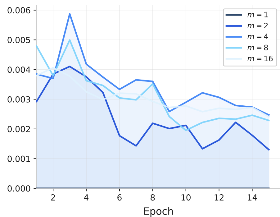
(c) C_8 — Orbit-Loss Variance
