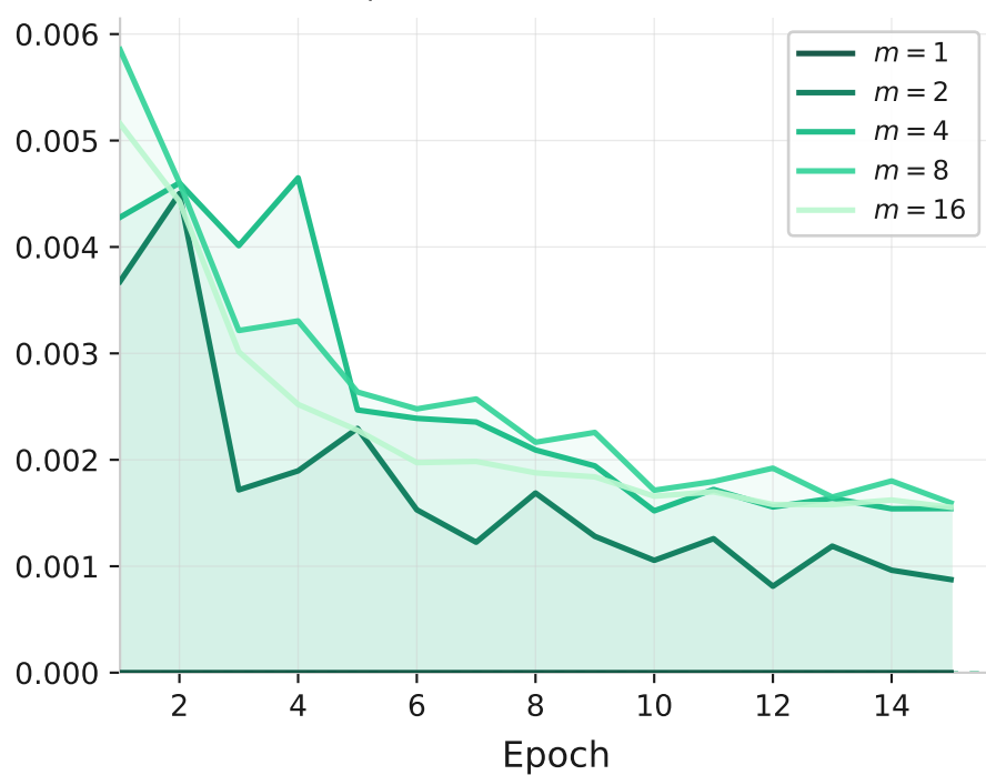
(b) C_4 — Orbit-Loss Variance
