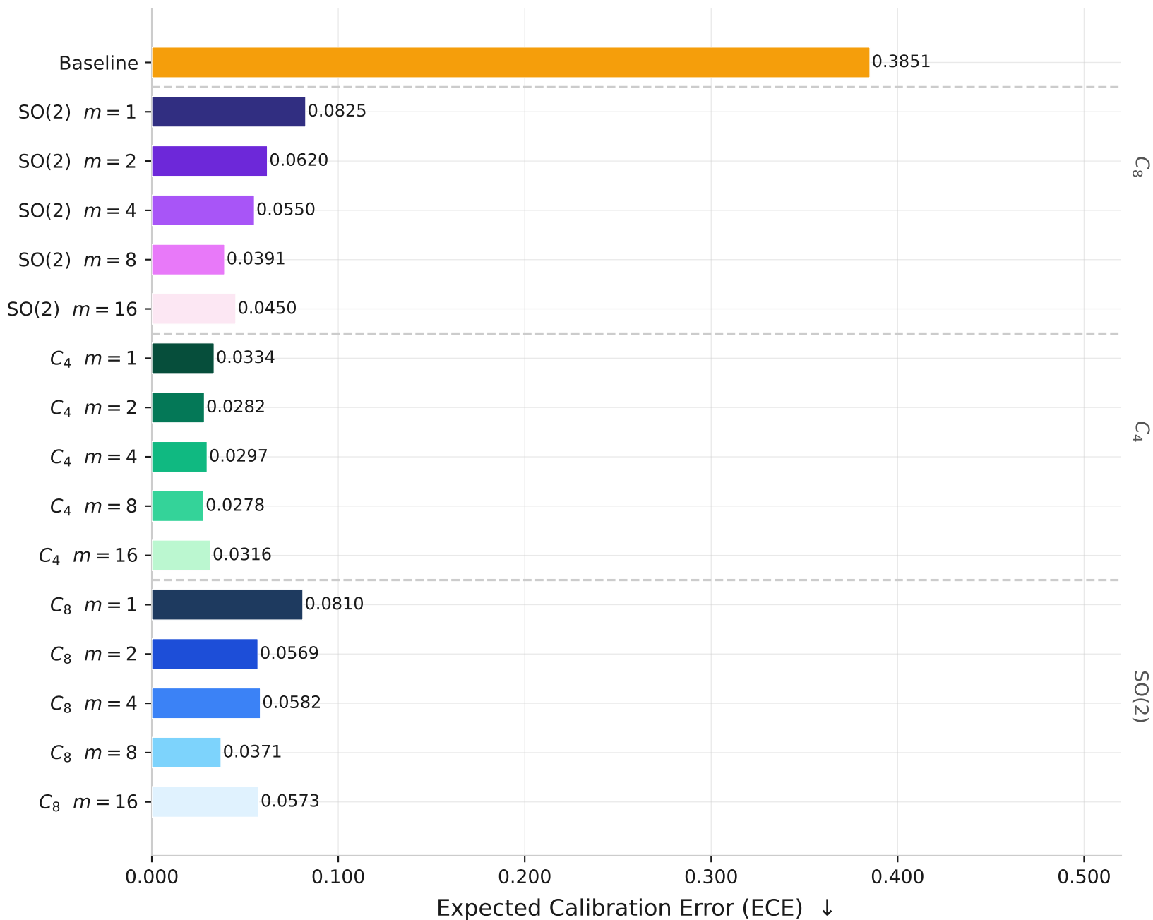
Expected Calibration Error by Augmentation Condition
