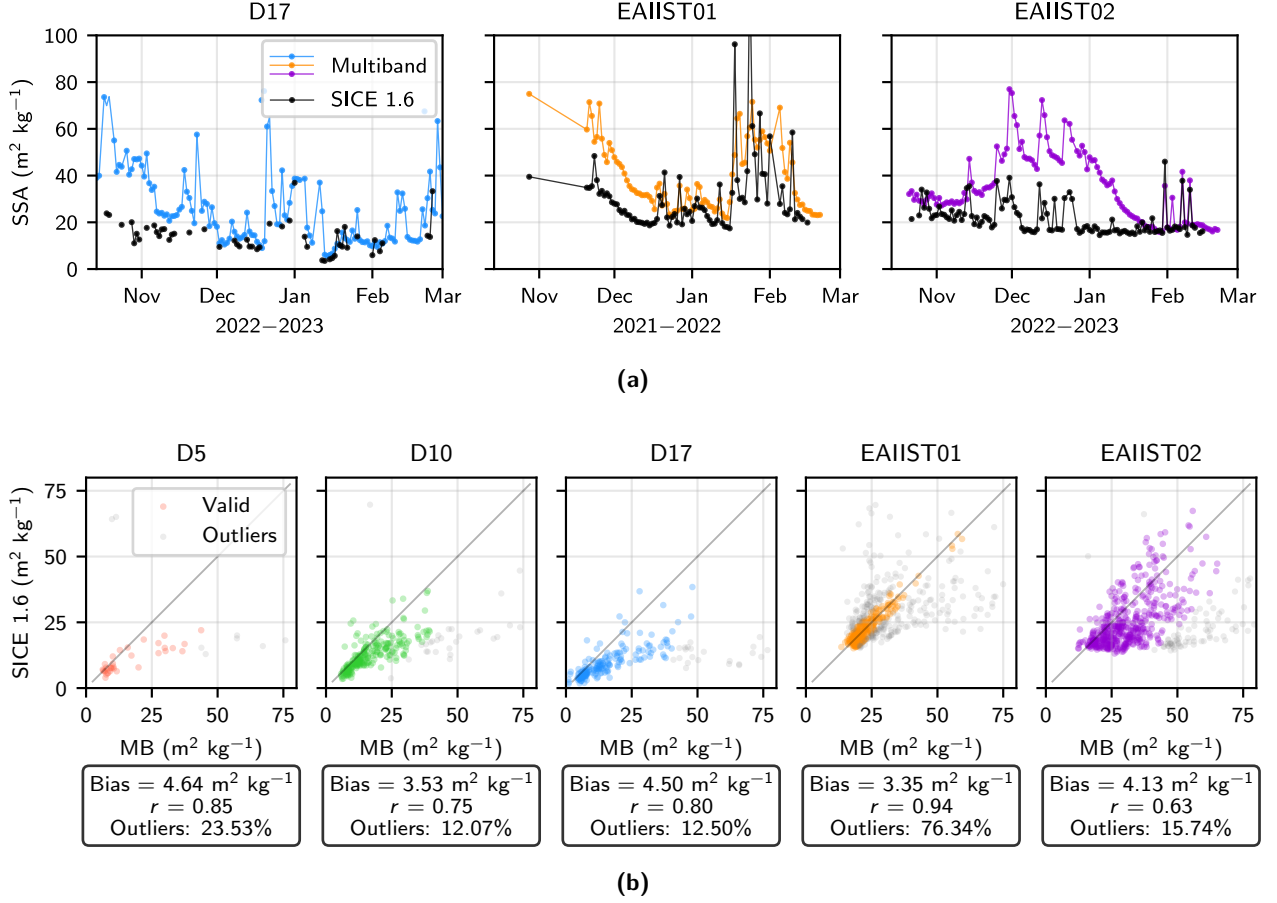
Figure 6: In situ and satellite retrieved SSAs | (a) Timeseries of SSA (top row) estimated from Multiband and from SICE 1.6 at D17 near Cap Prud’homme, EAIIST01 and EAIIST02 in the megadune (left to right) for selected austral summers (other years in Appendix); (b) comparison between SICE 1.6 and Multiband (bottom row) for the three Cap Prud’Homme stations and two megadunes stations. All statistics are computed exclusively on non-outliers and are significant at p < 0.01
