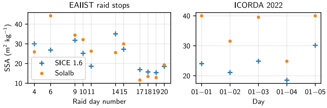
Figure 9: Cross-calibration experiment of EAIIST01 | Cgfkcalushdf
