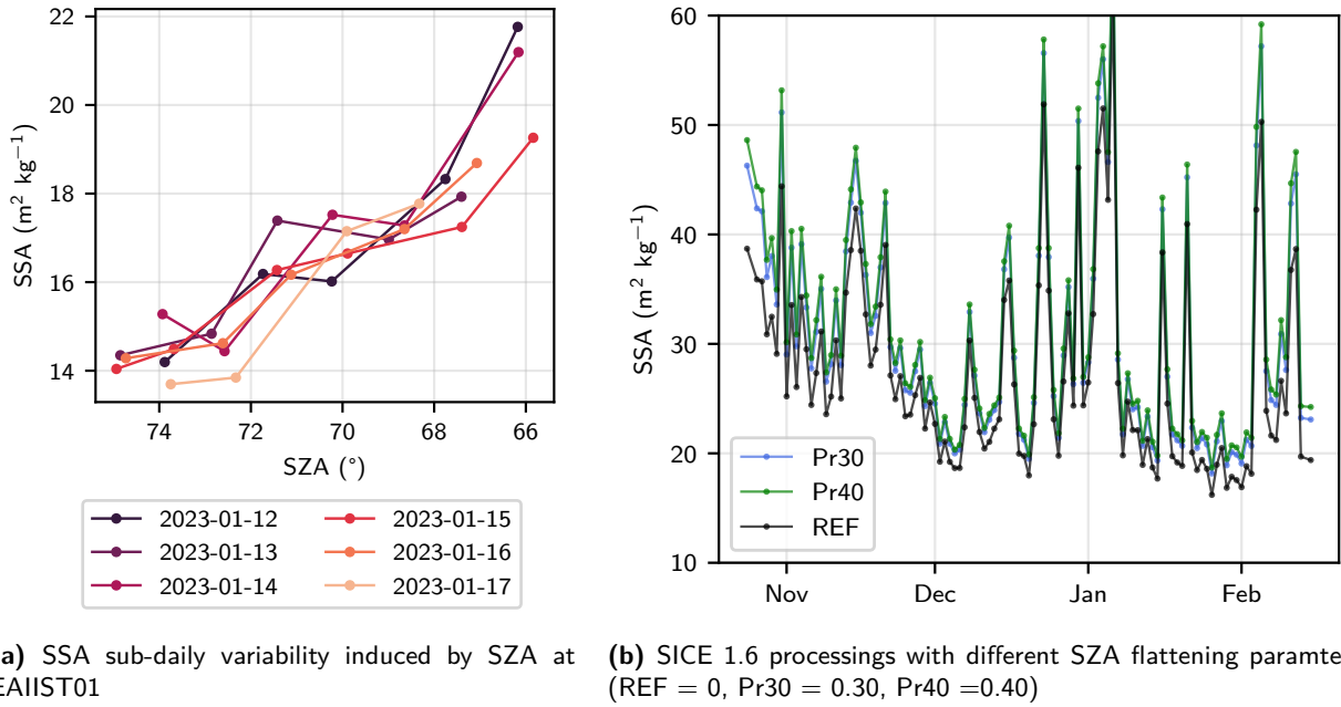
Figure 8: Diagnostic of SICE 1.6 | investigating the effect of SZA on grain size
