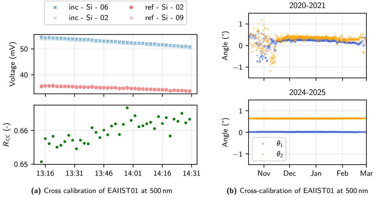
Figure 7: Calibrations and inclinometers | For both EAIIST stations
