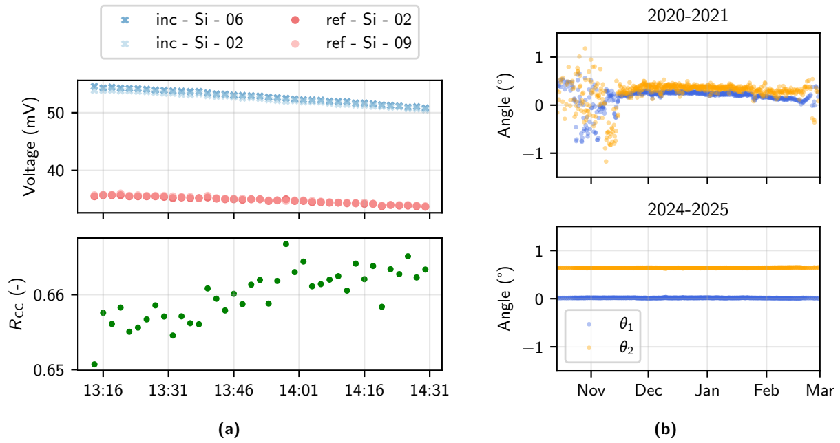
Figure 8: Calibrations and inclinometers | (a) Cross-calibration experiment performed for EAIIST01, carried on on December 29, 2019. In the upper plot, evolution of the raw signals at 500 nm: "inc" and "ref" are for incident and reflected channel respectively, "Si" is for the type of photodiode (Silicon), the digits 02, 06, 09 are the steps of the rotating wheel. In the lower plot, the ratio computed between the reflected and incident signals acquired at the same step (02). (b) Time series of the tilting angles measured by the inclinometer at EAIIST01 for two representative years.
