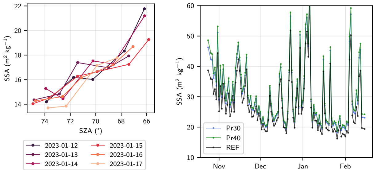
(a) SSA sub-daily variability induced by SZA at EAIIST01
