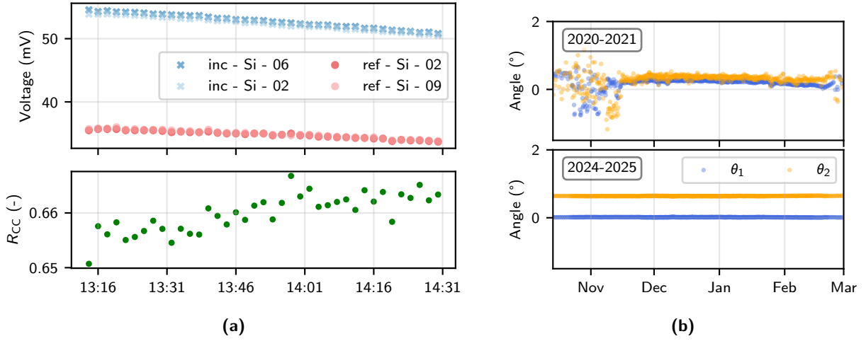
Figure 8: Calibrations and inclinometers | (a) Cross-calibration experiment performed for EAIIST01, carried on on December 29, 2019. In the upper plot, evolution of the raw signals at 500 nm: "inc" and "ref" are for incident and reflected channel respectively, "Si" is for the type of photodiode (Silicon), the digits 02, 06, 09 are the steps of the rotating wheel. In the lower plot, the ratio computed between the reflected and incident signals acquired at the same step (02). (b) Time series of the tilting angles measured by the inclinometer at EAIIST01 for two representative years.
