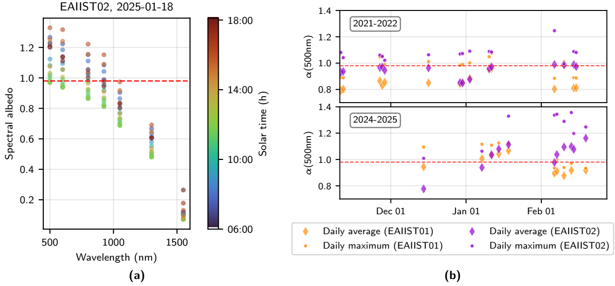
Figure 9: Multiband's albedo diagnostic | (a) Albedo spectra acquired during a mid-summer day with EAIIST02 albedometer. The dashed red line indicates the expected convergence value of the spectrum at 500 nm (0.98). (b) Interannual evolution of daily average (diamonds) and maximum spectral albedo (dots) at 500 nm at both EAIIST stations, during summer days with constant and diffuse light conditions only.
