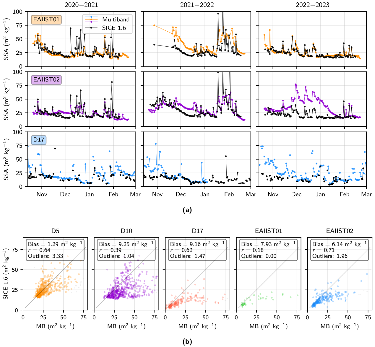
Figure 6: In situ and satellite retrieved SSAs | (a) Timeseries of SSA (top row) estimated from Multiband and from SICE 1.6 at D17 near Cap Prud'homme, EAIIST01 and EAIIST02 in the megadune (left to right) for selected austral summers (other years in Appendix); (b) comparison between SICE 1.6 and Multiband (bottom row) for the three Cap Prud'Homme stations and two megadunes stations. All statistics are computed exclusively on non-outliers and are significant at p < 0.01
