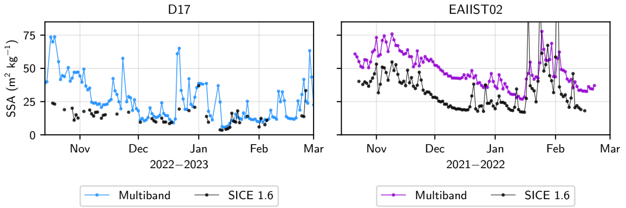
Figure 6: Representative SSA time series from Multiband and OLCI | On the left, data at D17 station at Cap Prud'homme; on the right, at EAIIST02 station in the megadunes zone
