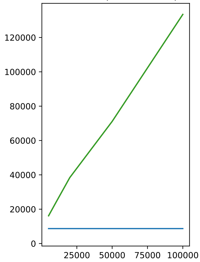
Domain PAC verifier, peak virtual space usage Domain AVE verifier, peak resident space
