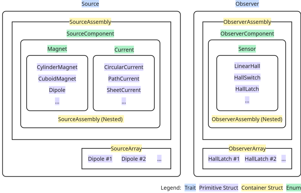
Figure 1: Core software architecture of the Magba library.
