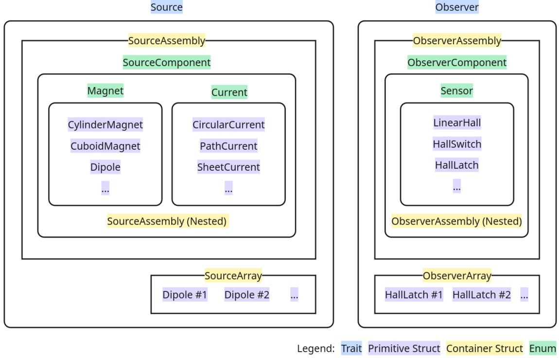
Figure 1: Core software architecture of the Magba library.
