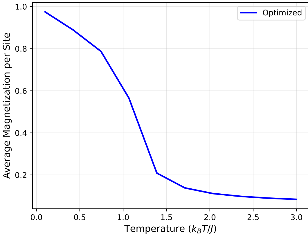
Magnetization vs Temperature (Optimized)
