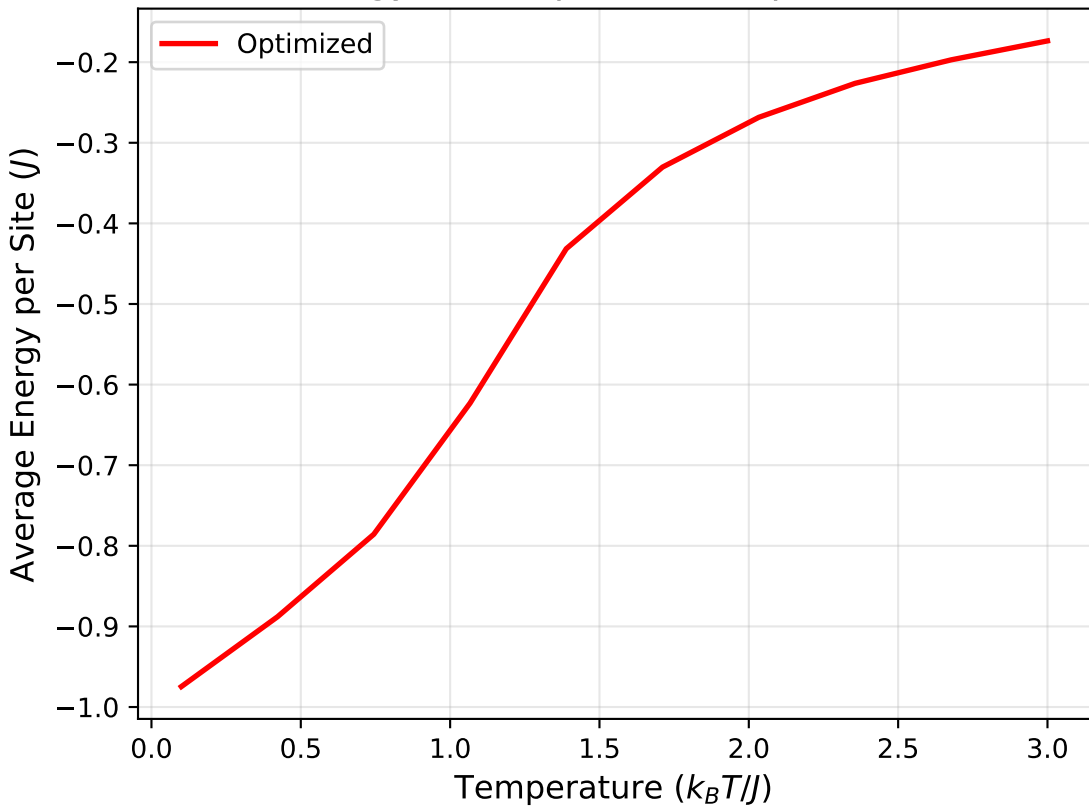
Energy vs Temperature (Optimized)
