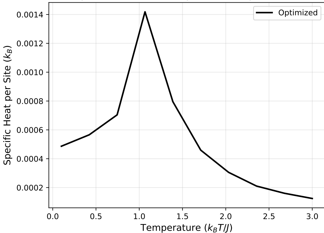
Specific Heat vs Temperature (Optimized)
