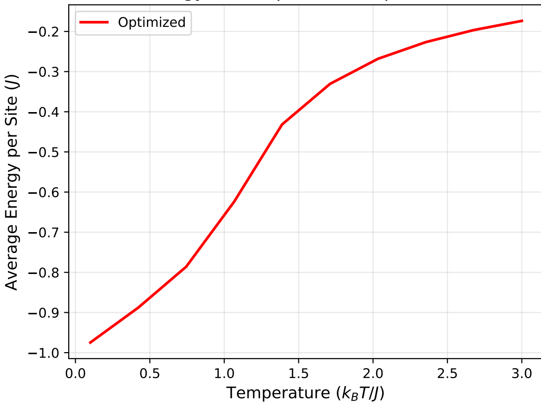
Energy vs Temperature (Optimized)
