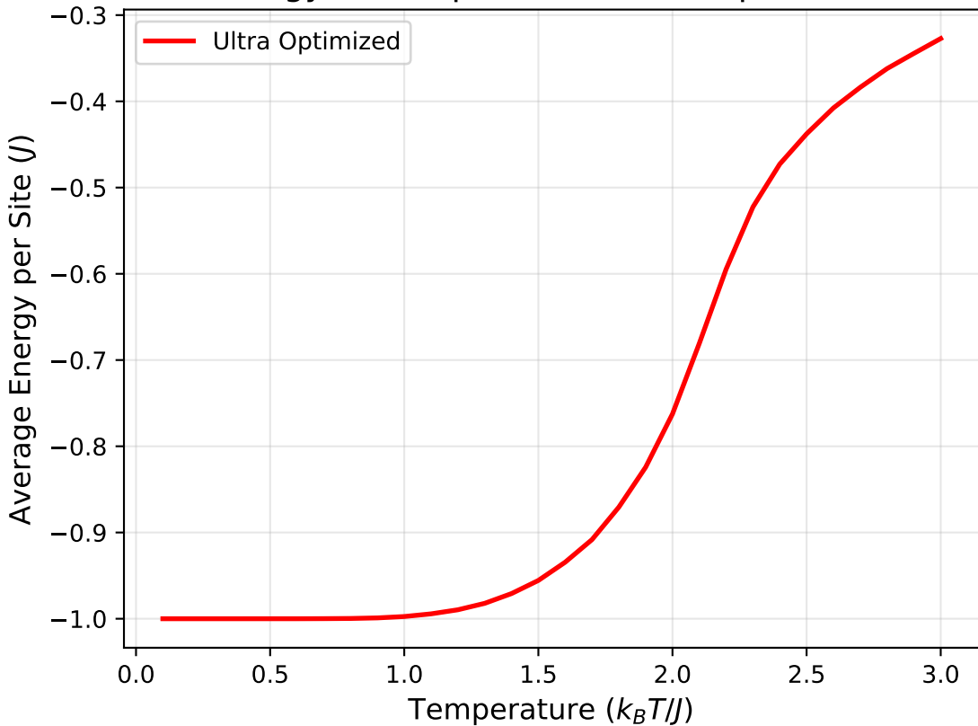
Energy vs Temperature (Ultra Optimized)
