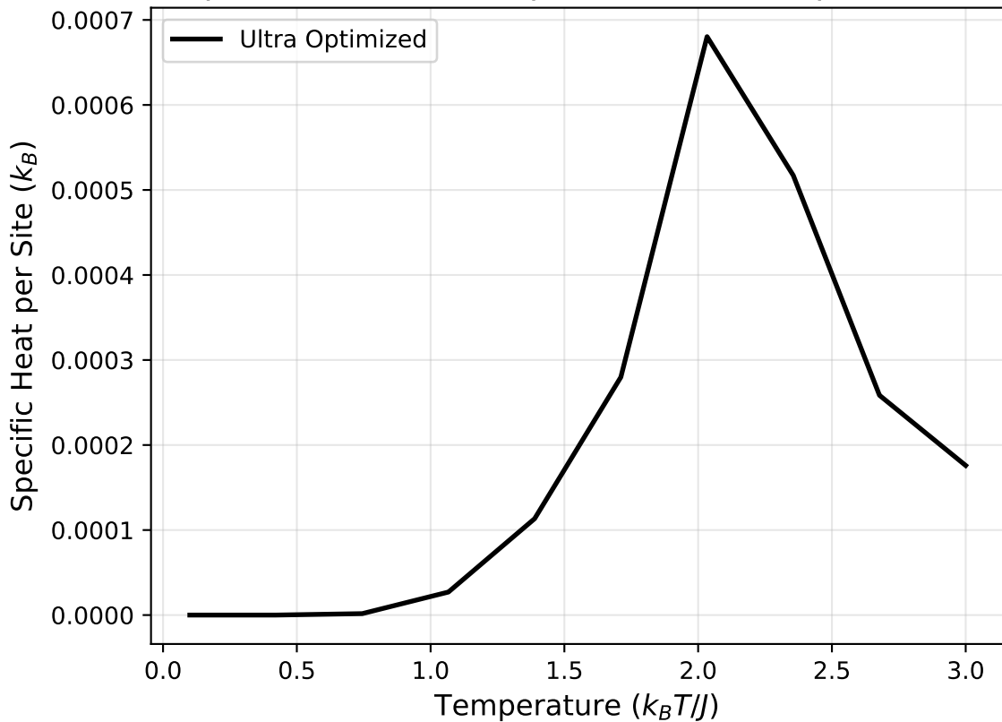
Specific Heat vs Temperature (Ultra Optimized)
