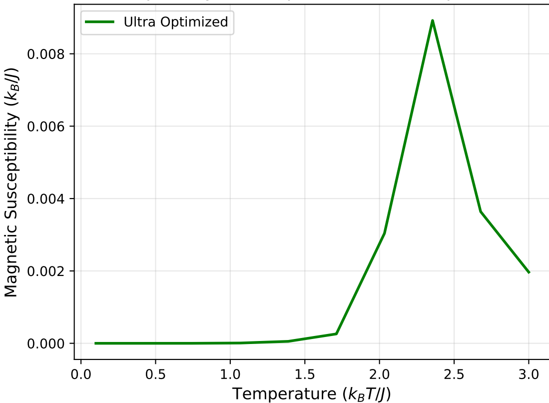
Susceptibility vs Temperature (Ultra Optimized)
