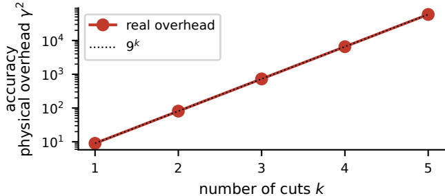
(b) qiskit-addon-cutting: overhead = 9^k
