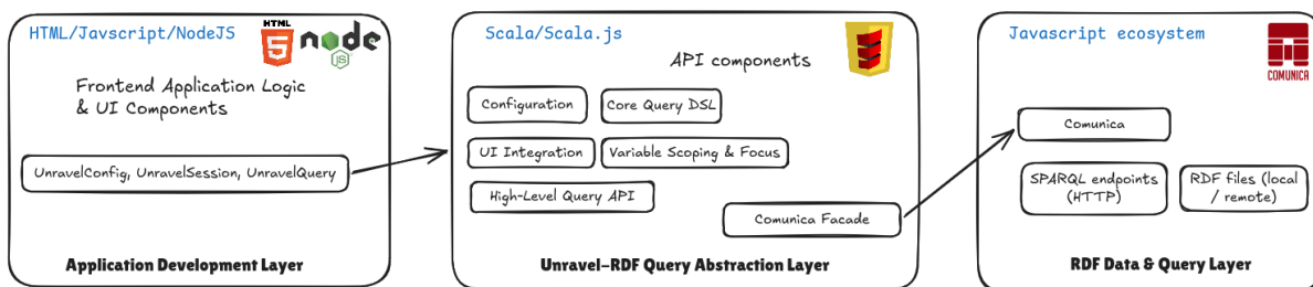
Figure 1: Unravel-RDF architecture: a layered design connecting RDF data sources, the Unravel query abstraction layer, and UI integration components.
