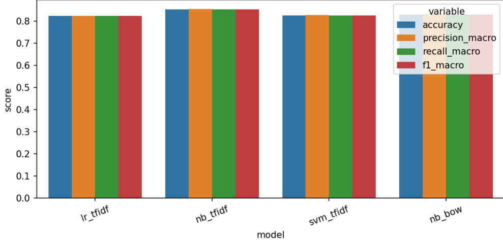
Figure 1: Aggregate test-set metrics across the four pipelines. Multinomial Naïve Bayes on TF-IDF dominates every metric.
