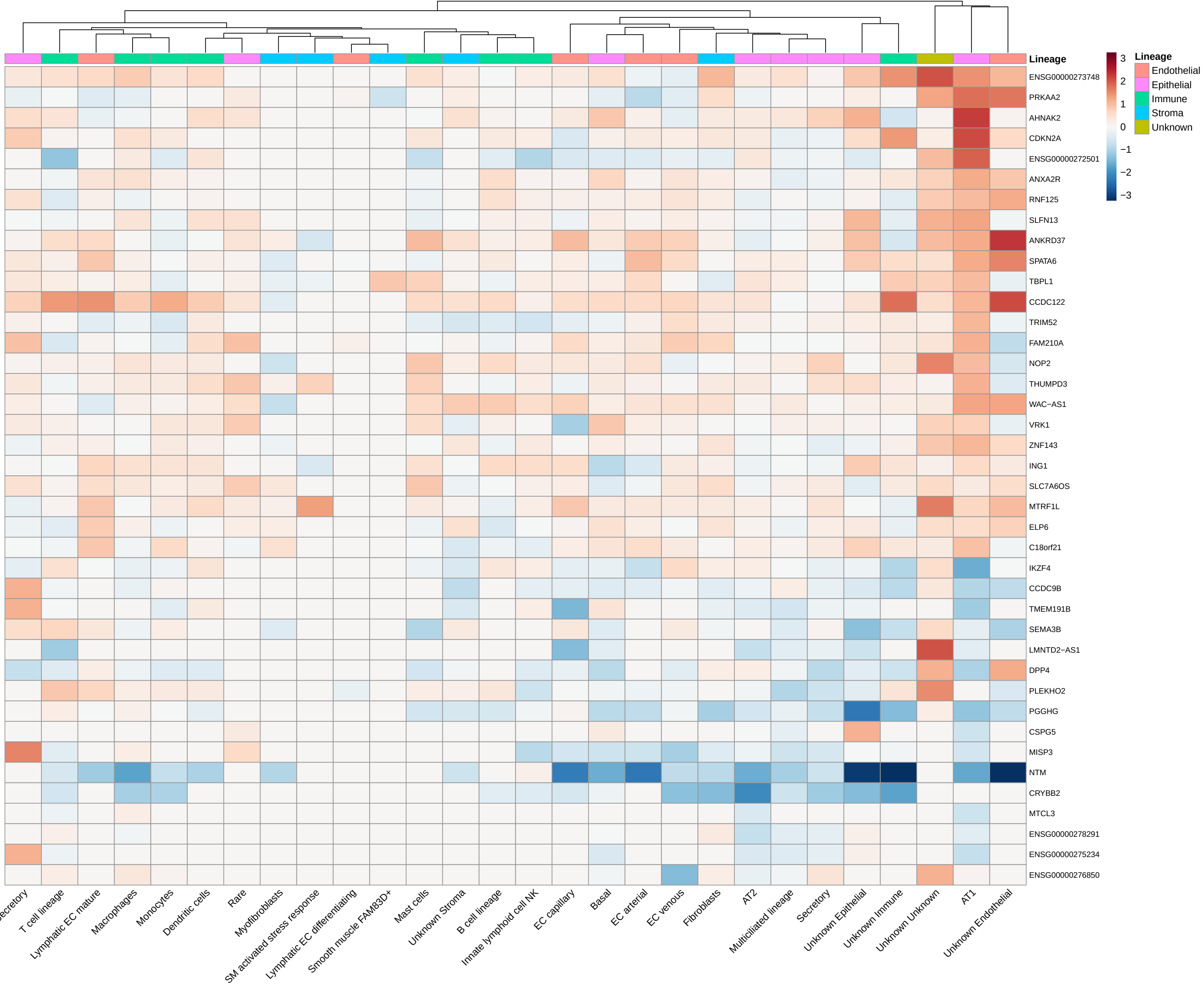
Age logFC (Old vs Young): top genes x cell type
