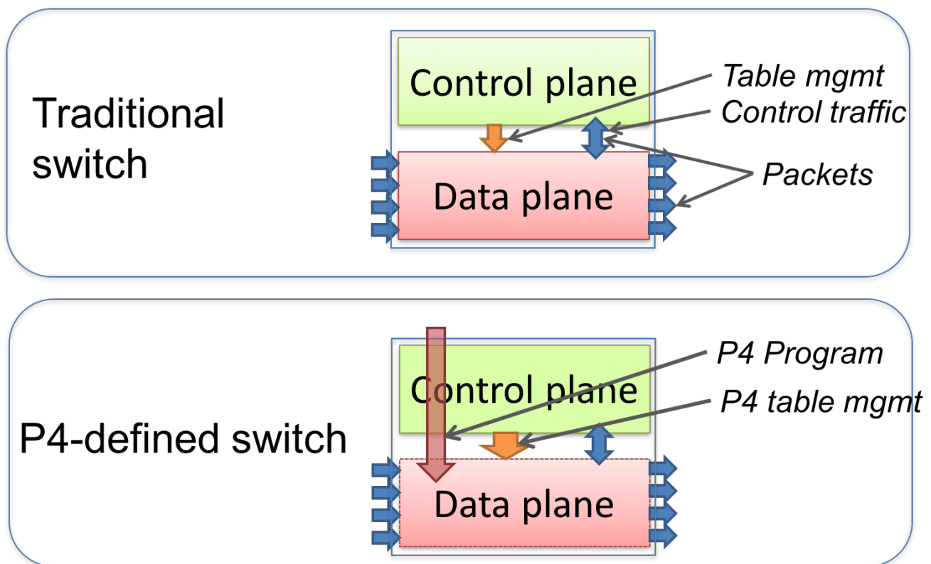
Figure 1. Traditional switches vs. programmable switches.
