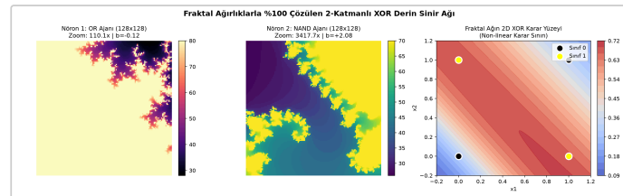
Fig. 5. Complete 2-layer composite fractal neural network resolving the non-linear XOR problem with 100% accuracy, generating a continuous non-linear 2D classification boundary.
