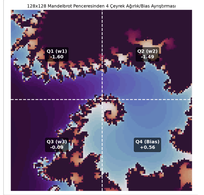
Fig. 2. 4-Quadrant Partitioning on a 128 \times 128 window. Non-escaping black pixel ratios in sub-regions (Q 1 , Q 2 , Q 3 , Q 4 ) yield independent synaptic weights ( w_1, w_2, w_3 ) and neuron bias (b).
