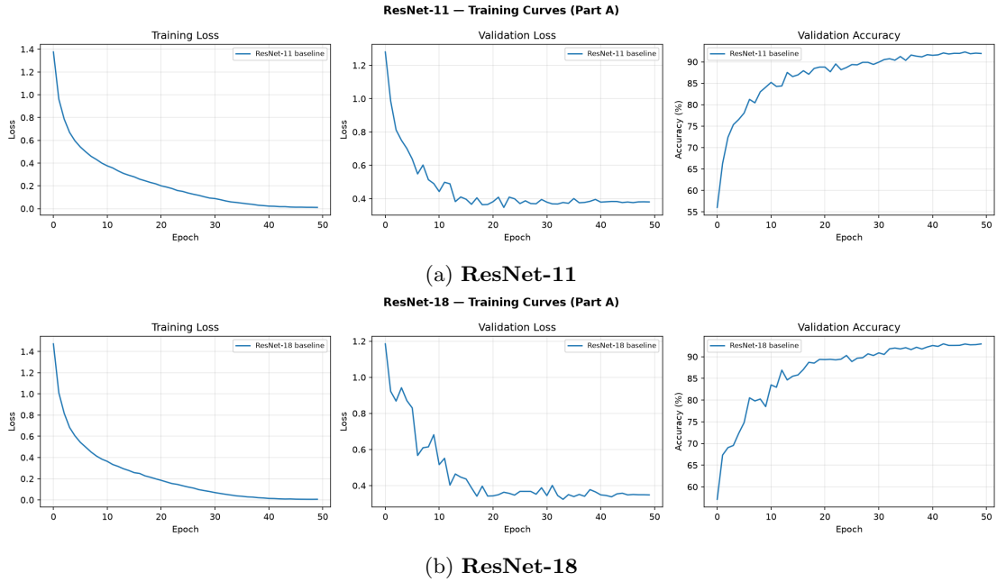
Figure 14: Training Curves for Part A for both models
