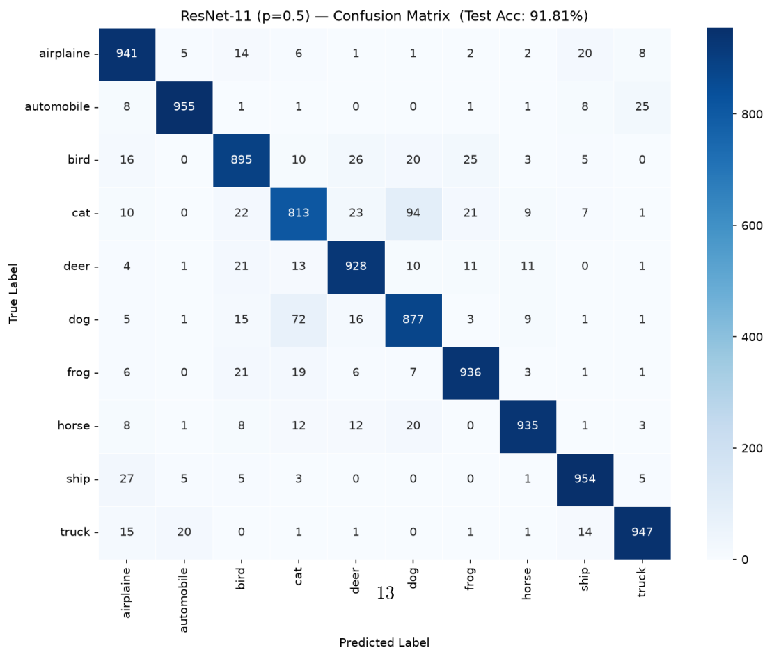
(b) Drouput = 0.5
