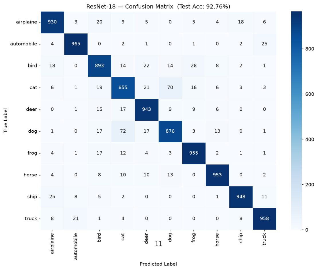
(b) ResNet-18
