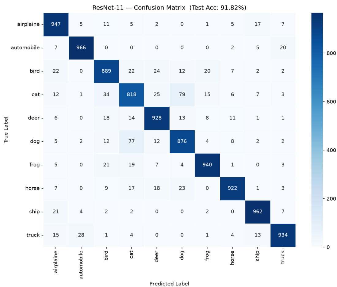
(a) ResNet-11
