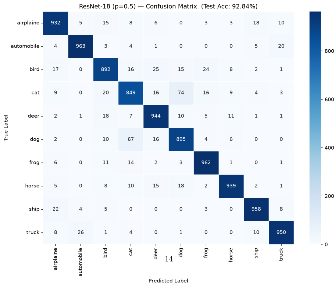
(b) Drouput = 0.5
