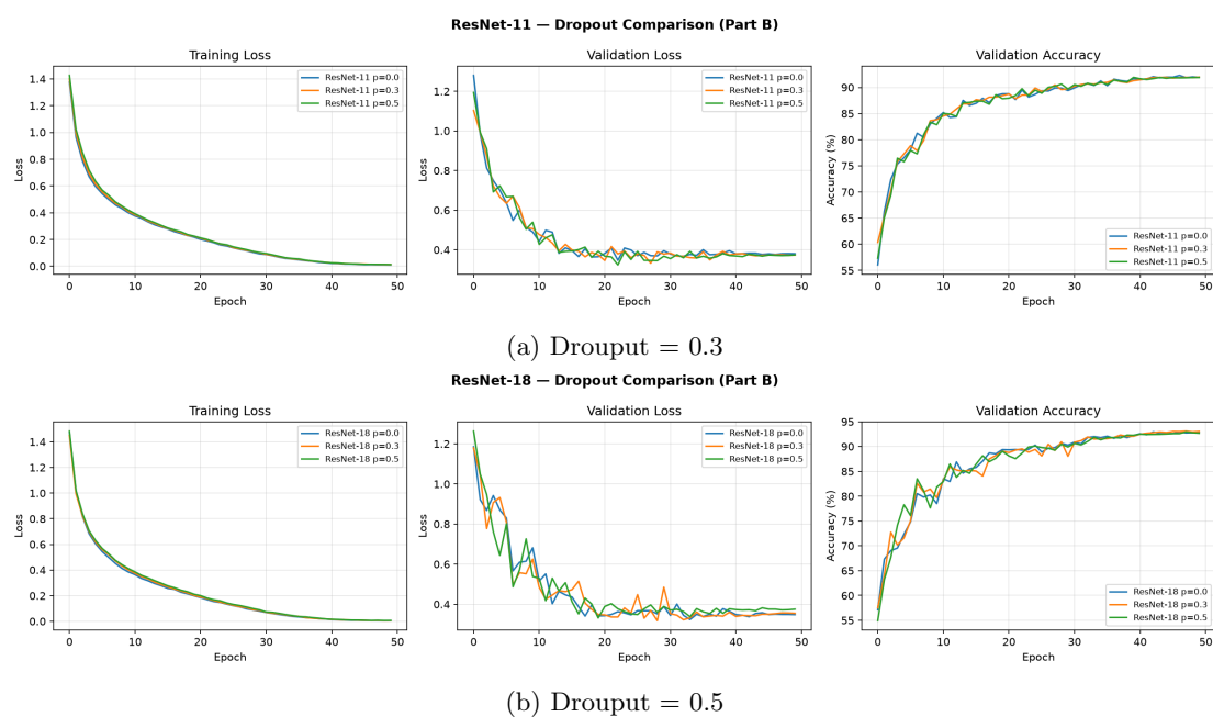
Figure 19: Training Curves for Different Dropouts of ResNet Models
