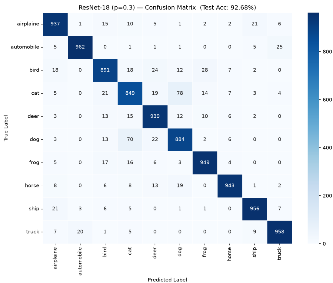
(a) Drouput = 0.3
