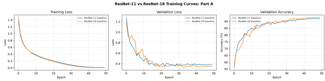
Figure 16: Comparison between ResNet Models
