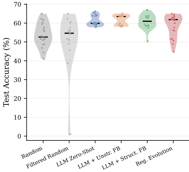
CIFAR-100
