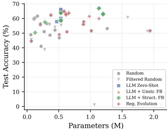
CIFAR-100
