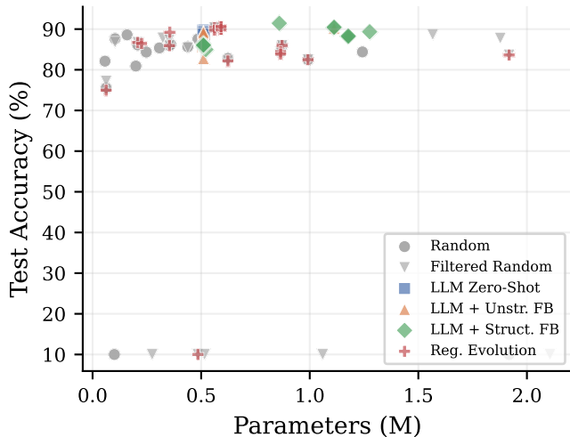
CIFAR-10
