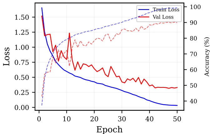
LLM (Unstructured FB) (Best: 89.8%, 723K params)
