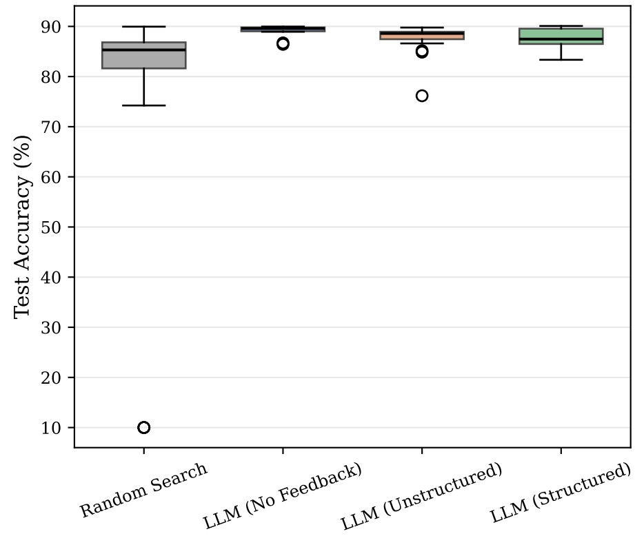
CIFAR-10
