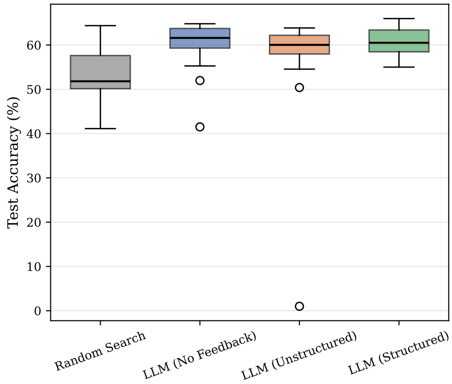
CIFAR-100
