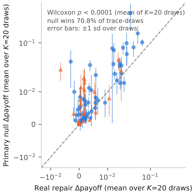
B. Experiment 2: corrected payoff
