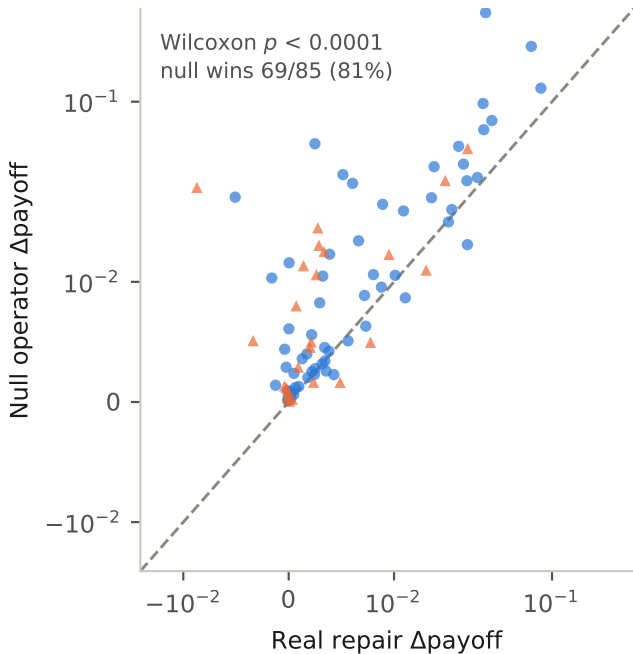
A. Experiment 1: original payoff
