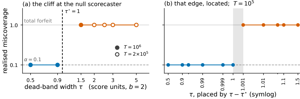
Figure 2: Realised miscoverage against dead-band width \tau at the null scorecaster, \hat{q} \equiv 0 with a saturator of level b , where \tau^* = \sup_x r_t(x) + \sup_t \hat{q}_t - b/2 is 1. (a) The full sweep: filled markers run to T = 10^6 and the four widest bands, drawn open, to T = 2 \times 10^5 ; blue covers, orange forfeits, and the dashed rule is \tau^* . (b) The same setting at T = 10^5 over eleven measured widths, placed by \tau - \tau^* on a symlog axis whose linear zone is |\tau - \tau^*| \leq 10^{-3} , each tick carrying the \tau it marks. The grey band spans the widest covering width to the narrowest failing one; Figure 3 gives the other four (r_t, \hat{q}) settings.
