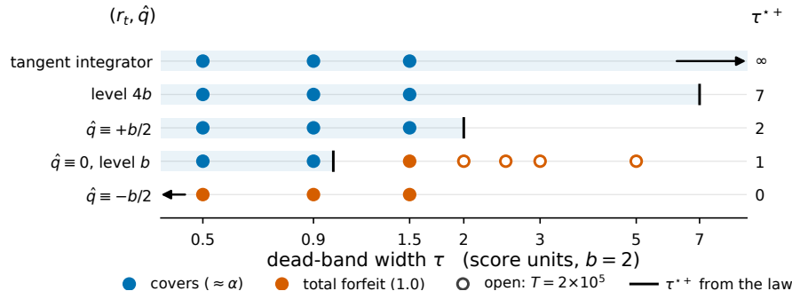
Figure 3: All 19 dead-band runs, at the five admissible (r_t, \hat{q}) settings: rows are settings ordered by \tau^* , and the shared horizontal axis is \tau . Blue markers cover at \approx \alpha and orange markers return 1.000000; filled markers run to T = 10^6 and open markers to T = 2 \times 10^5 , all under the specified adversary. The rule on each row is that setting's upward boundary \tau^{*+} = \sup_x r_t(x) + \sup_t \hat{q}_t - b/2 , printed at the right, and the tinted band is \tau \leq \tau^{*+} . Two rules fall off the axis and are drawn as arrows: \tau^{*+} = 0 at \hat{q} \equiv -b/2 , and \tau^{*+} unbounded under Angelopoulos et al.'s tangent integrator. The mirror boundary \tau^{*-} of (2) is not drawn here and differs from \tau^{*+} at the two non-null scorecasters.
