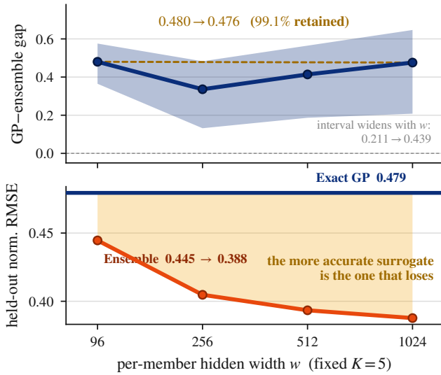
Figure 3: The two eliminations that rule out capacity and accuracy, in one image. Top: at fixed K=5 the GP-ensemble gap does not close over a 10.7\times width sweep ( 0.480 \rightarrow 0.476 ); the curve is non-monotone, and the bootstrap band widens with w , so w=1024 is the least precise point on it—a limit we state rather than smooth over. Bottom: the ensemble’s held-out normalized RMSE falls monotonically with width and lies below the exact GP’s flat line at every width. The more accurate surrogate is the one that loses. Synthetic grid, 7 tasks, 30 seeds, B=10,000 ; RMSE on a 20% split the grid never saw.
