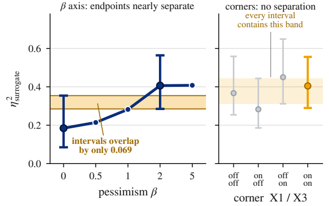
Figure 3: The \beta axis is the one these seven tasks come closest to resolving, and the engine corners are the one they cannot resolve at all. Left: \eta_{\text{surr}}^2 rises monotonically with pessimism, and the \beta=0 and \beta=2 intervals overlap by only 0.069. Intervals were computed at those two endpoints and are drawn nowhere else. Right: on the same scale, the four corner intervals overlap completely, sharing a common region every one of them contains. This is why the paper leads its decomposition with \beta and never asserts a corner difference. Synthetic grid, 7 tasks, 30 seeds, B=10,000 .
