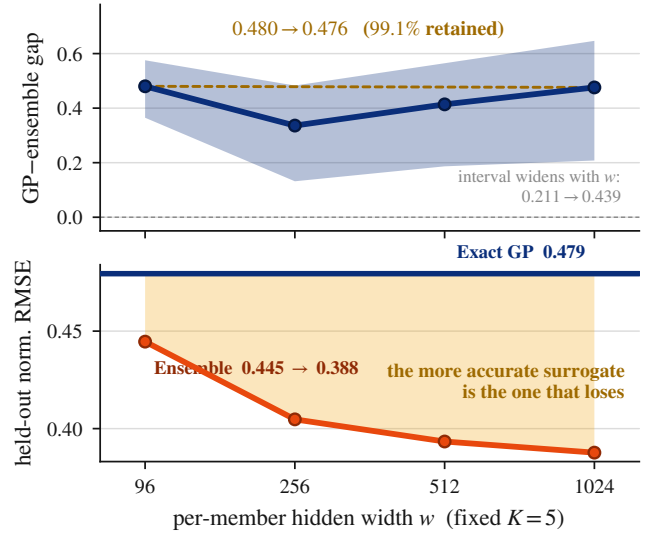
Figure 4: The two eliminations that rule out capacity and accuracy, in one image. Top: at fixed K=5 the GP-ensemble gap does not close over a 10.7\times width sweep ( 0.480 \rightarrow 0.476 ); the curve is non-monotone, and the bootstrap band widens with w , so w=1024 is the least precise point on it—a limit we state rather than smooth over. Bottom: the ensemble’s held-out normalized RMSE falls monotonically with width and lies below the exact GP’s flat line at every width. The more accurate surrogate is the one that loses. Synthetic grid, 7 tasks, 30 seeds, B=10,000 ; RMSE on a 20% split the grid never saw.
