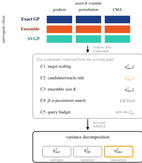
Figure 1: The design: a crossed surrogate \times optimizer factorial—three surrogate classes against three search routines under one shared protocol—from which five confounds specific to offline-MBO surrogate comparison are removed (each traced to a line of the scoring path, each with a signed effect), then decomposed by two-way ANOVA into the surrogate and optimizer main effects and the surrogate \times optimizer interaction the factorial exists to estimate.
