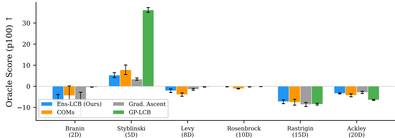
Offline MBO: 100th Percentile Oracle Score (6 tasks, higher is better)
