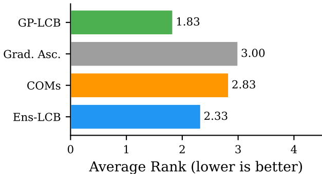
Average Rank (6 tasks)
