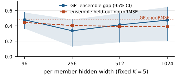
Figure 2: Two eliminations in one image. At fixed K=5 the gap is flat with noise across a 10.7\times width range (intervals widen with w : the claim is that the gap does not close, not that it is identical), while the ensemble’s held-out normRMSE falls monotonically and overtakes the GP’s.
