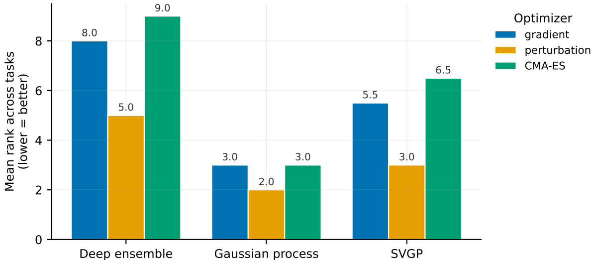
Acquisition optimizer decides ensemble performance, but barely matters for GP surrogates
