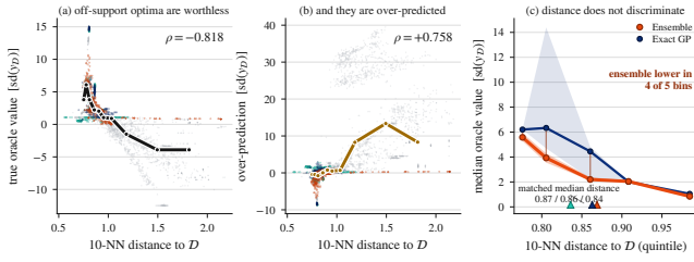
Figure 3: Distance predicts worthlessness (a, \rho = -0.818 ) and over-prediction (b, \rho = +0.758 ) across all 5,040 returned optima but does not discriminate between surrogate classes (c): at matched median distance (0.87/0.86/0.84) the ensemble is still lower in oracle value, in four of five bins. Panel (c) is ensemble against exact GP (SVGP omitted, its distance-value bootstrap correlation near zero); bands are 95% bootstrap intervals on the bin median. Audited engine, X1/X3 on, \beta=2 , K=5 .
