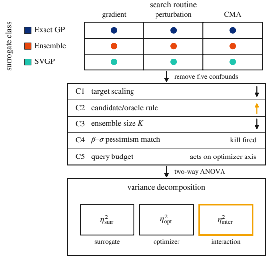
Figure 1: The design: a crossed surrogate \times optimizer factorial (three surrogate classes, three search routines, one shared protocol), five confounds specific to offline-MBO surrogate comparison removed, then decomposed by two-way ANOVA into the two main effects and the interaction the factorial exists to estimate.
