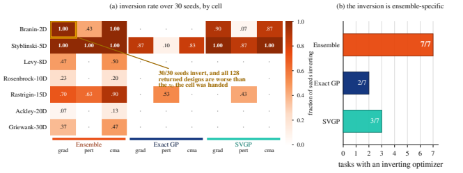
Figure 4: The ensemble’s LCB ranks designs it invented above real designs it was handed. (a) Inversion rate over 30 seeds, all 63 cells: the ensemble block lights up, the exact GP’s stays dark. (b) Tasks with at least one inverting optimizer: 7/7 ensemble, 3/7 SVGP, 2/7 exact GP. Audited engine, X1/X3 on, K=5 , \beta=2 , 30 seeds.
