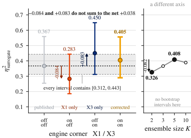
Figure 1: The four engine corners as measured levels, not as a composing cascade. Target scaling alone (X1) moves \eta^2_{\text{surrogate}} down 0.084 and the candidate/oracle rule alone (X3) moves it up 0.083, but the corner where both are applied sits 0.038 above the uncorrected one: the corrections are not additive , and the corrected 0.405 [0.290, 0.556] is a measured joint level rather than a sum of the separate effects, which very nearly cancel. The shaded band is the region every corner’s bootstrap interval contains—the four intervals overlap so heavily that no corner is separable from another at n=7 , which is the pre-registered KB5 result. What this figure localizes is therefore the signed direction of each correction, never an additive budget and never a corner-to-corner difference. Ensemble size sits in a separate panel because it is a confound on a different axis, not a fifth corner; its sweep was not bootstrapped, so those points carry no intervals. Confounds 4 and 5 are absent by measurement, not omission: Confound 4’s aggregate kill criterion fired, so it has no grid-wide \eta^2_{\text{surrogate}} effect, and Confound 5 acts on \eta^2_{\text{opt}} . Synthetic grid, n=7 tasks, 30 seeds, B=10,000 bootstrap.
