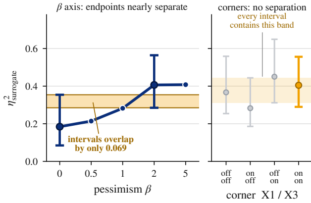
Figure 2: The \beta axis is the one these seven tasks come closest to resolving, and the engine corners are the one they cannot resolve at all. Left: \eta^2_{\text{surr}} rises monotonically with pessimism, and the \beta=0 and \beta=2 intervals overlap by only 0.069. Intervals were computed at those two endpoints and are drawn nowhere else. Right: on the same scale, the four corner intervals overlap completely, sharing a common region every one of them contains. This is why the paper leads its decomposition with \beta and never asserts a corner difference. Synthetic grid, 7 tasks, 30 seeds, B=10,000 .
