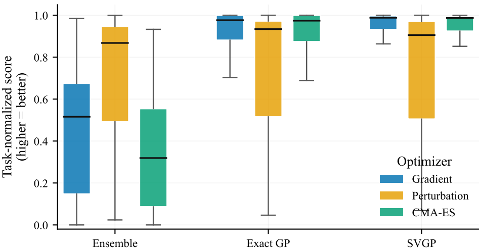
The acquisition optimizer swings ensemble outcomes but is nearly inert for calibrated posteriors
