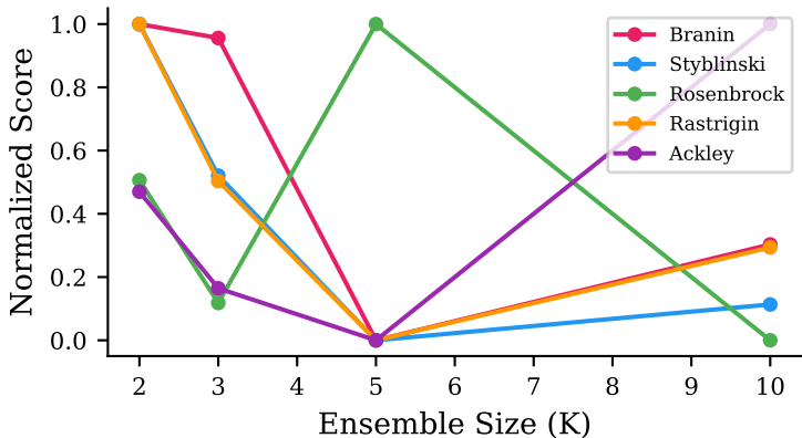
Ensemble Size Ablation
