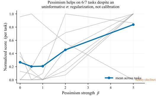
Figure 6: Pessimism sweep: per-task normalized 100th-percentile score vs. \beta (faint lines, individual synthetic tasks; bold line, mean). Score rises with \beta on 6 of 7 tasks even though \sigma is an uninformative error signal ( \rho \approx 0.1 )—pessimism acts as distance-regularization. Ackley is the single task where the penalty points the wrong way.
