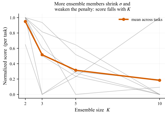
Figure 2: Ensemble-size ablation. Task-normalized score decreases with K .
