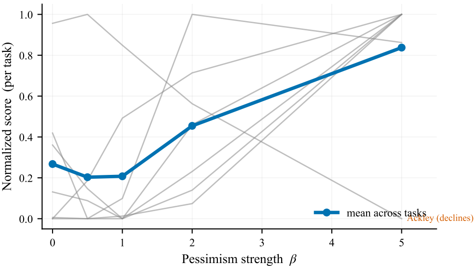
Pessimism helps on 6/7 tasks despite an uninformative \sigma : regularization, not calibration
