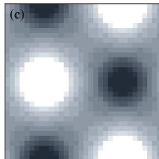
gyroid
