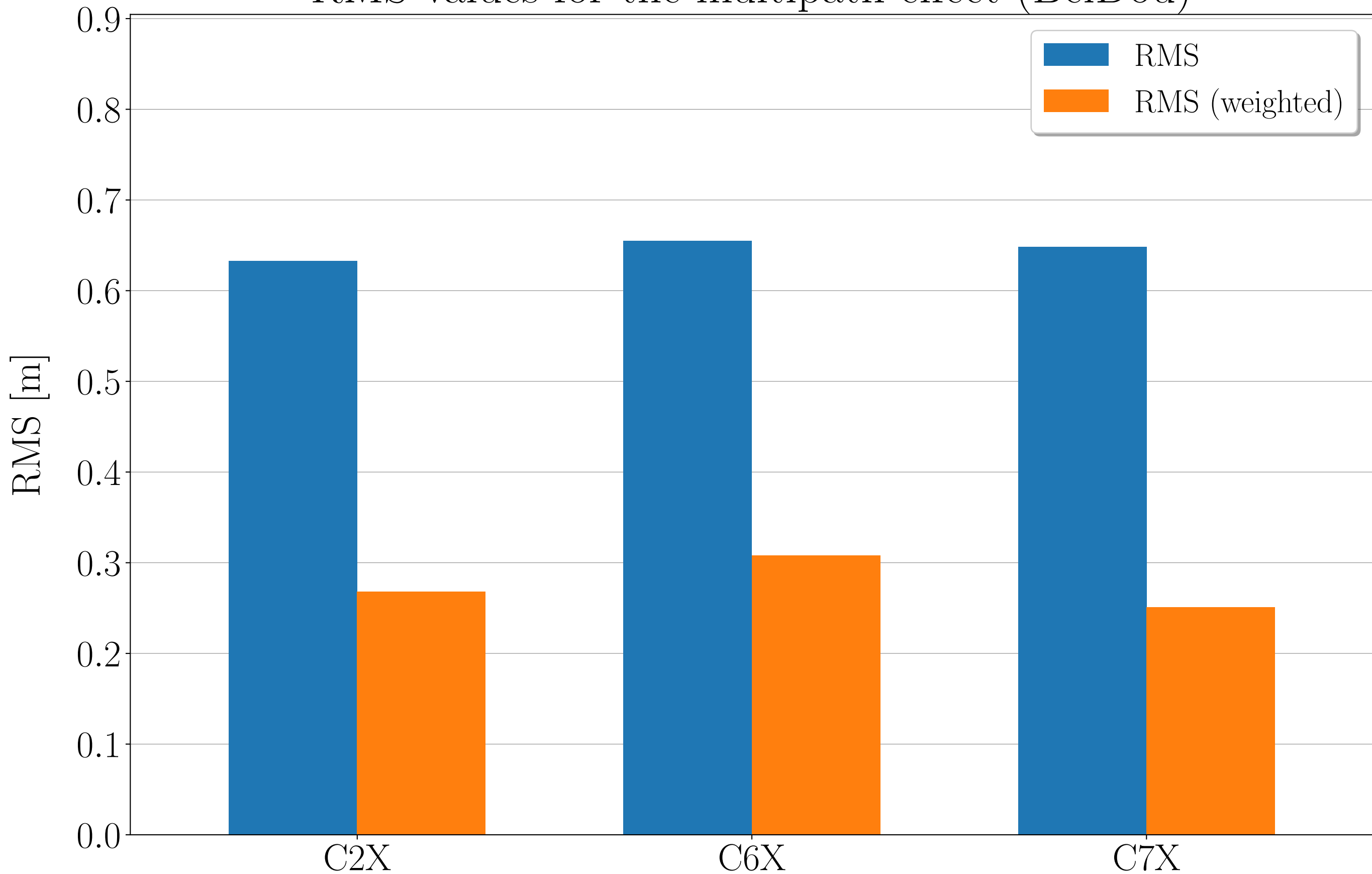
RMS values for the multipath effect (BeiDou)
