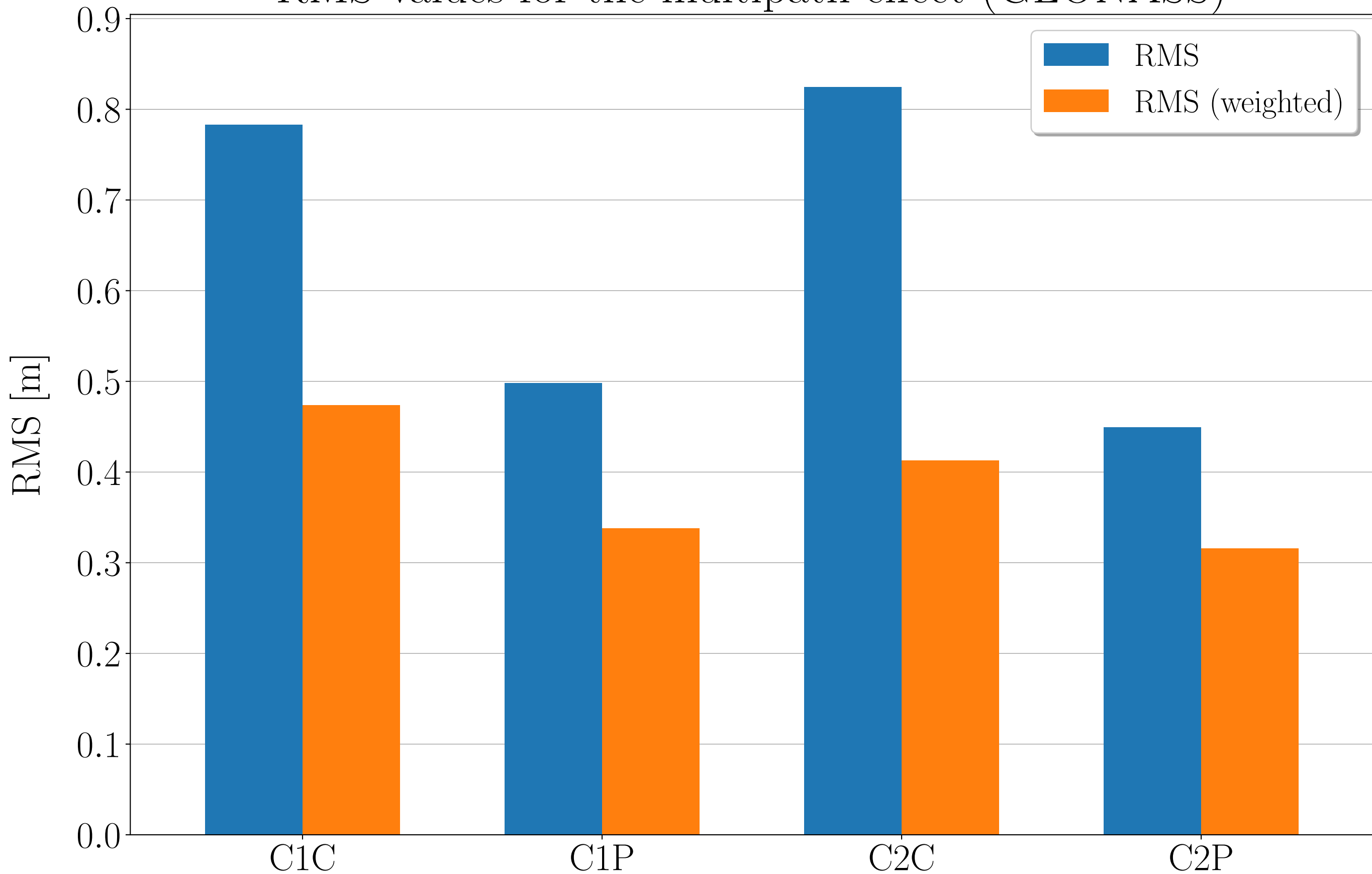
RMS values for the multipath effect (GLONASS)
